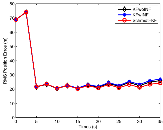
Figure 1: Position RMSE for target with GMTI measurement (moderate bias, OOSM processing).
